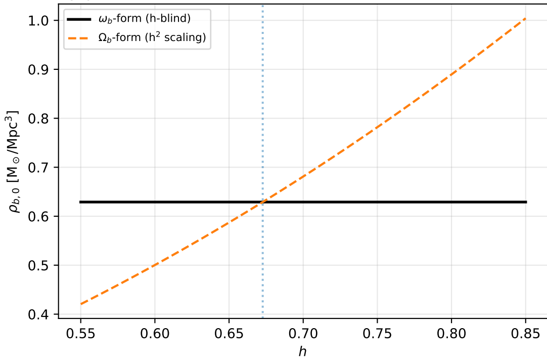
h-blindness of \rho_{b,0} in \omega_b variables (Thm 1, C1)
