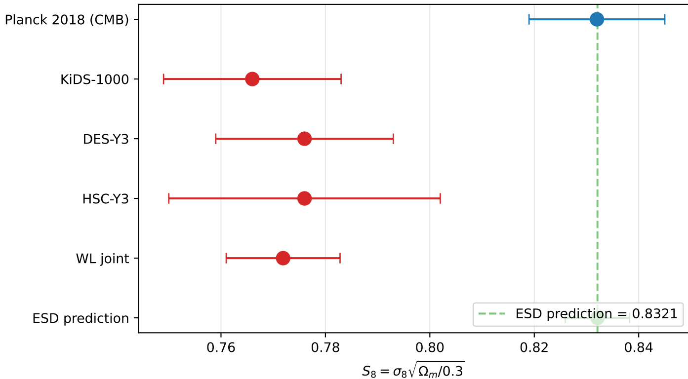
ESD predicts S_8 = 0.832 (Planck-side) from \sigma_8 + \text{locked } \Omega_m
