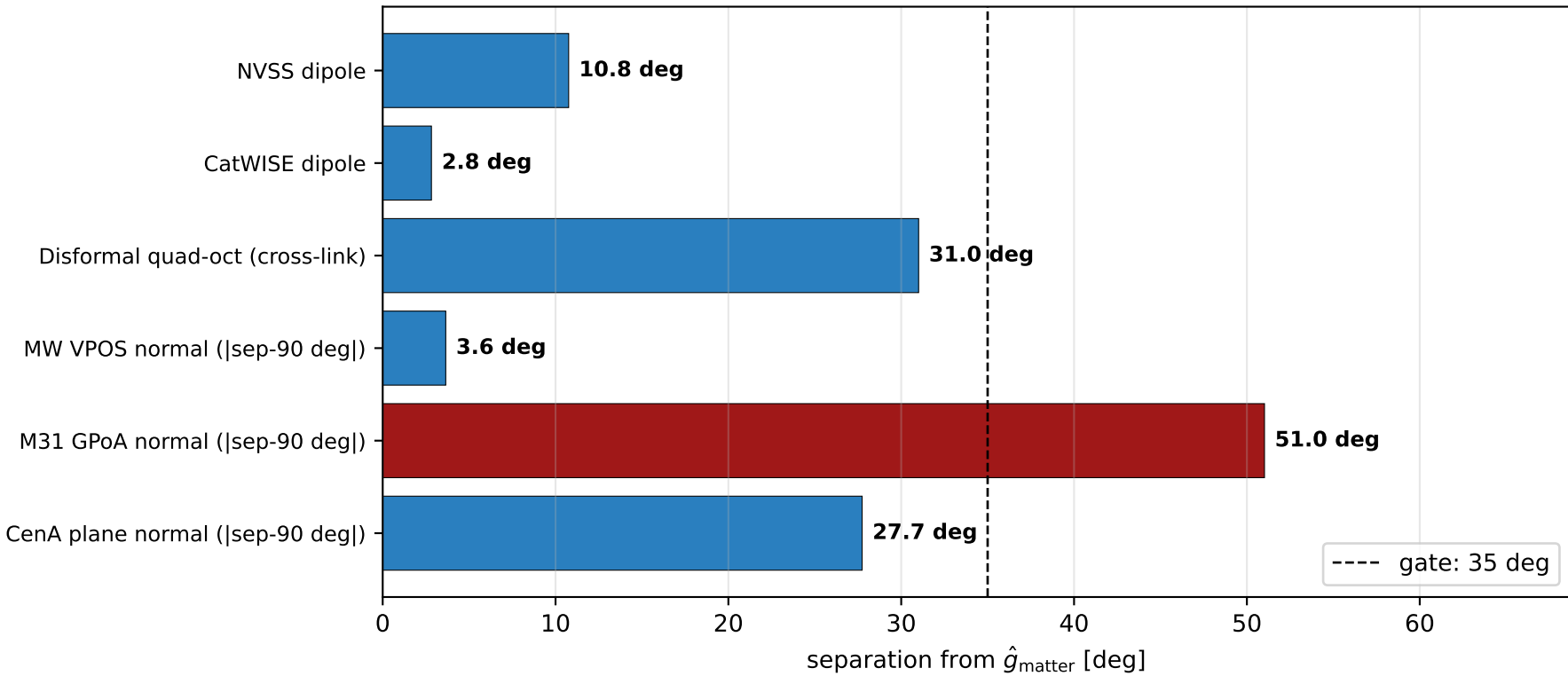
Study 25 - MATTER channel cross-observable alignment (5/6 PASS)
