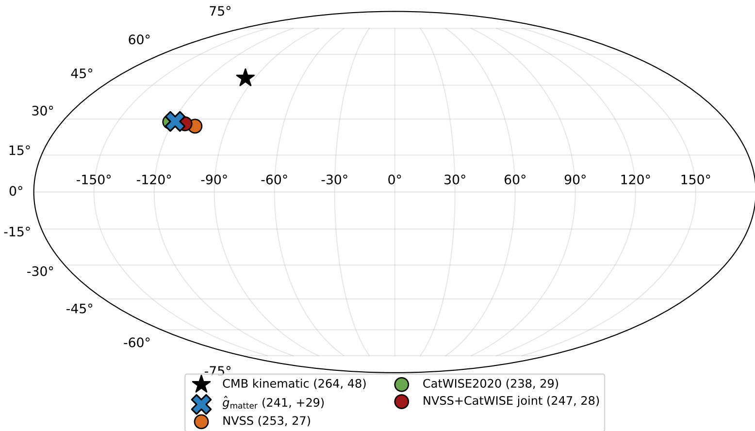
Cosmic dipole axes vs MATTER-channel \hat{g} (galactic)
