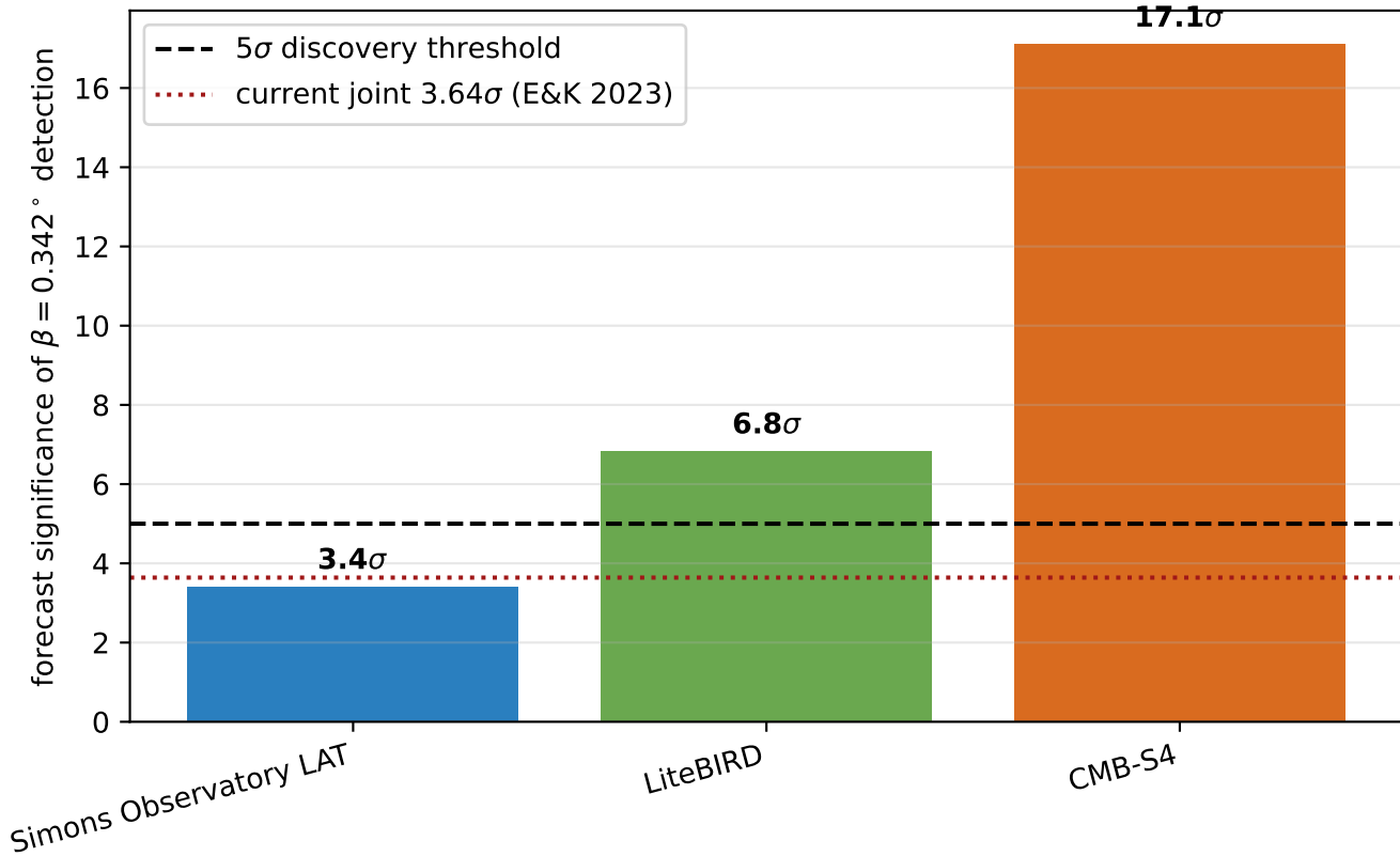
Study 26 - Falsifier forecast for ESD's \beta = 0 prediction
