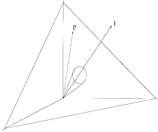
Fig. 1. Schematic view of the situation in which function space \mathcal{F} is three dimensional. The uniform prior over this space, \mathbf{l} , lies along the diagonal. Different algorithms a give different vectors v lying in the cone surrounding the diagonal. A particular problem is represented by its prior \mathbf{p} lying on the simplex. The algorithm that will perform best will be the algorithm in the cone having the largest inner product with \mathbf{p} .
