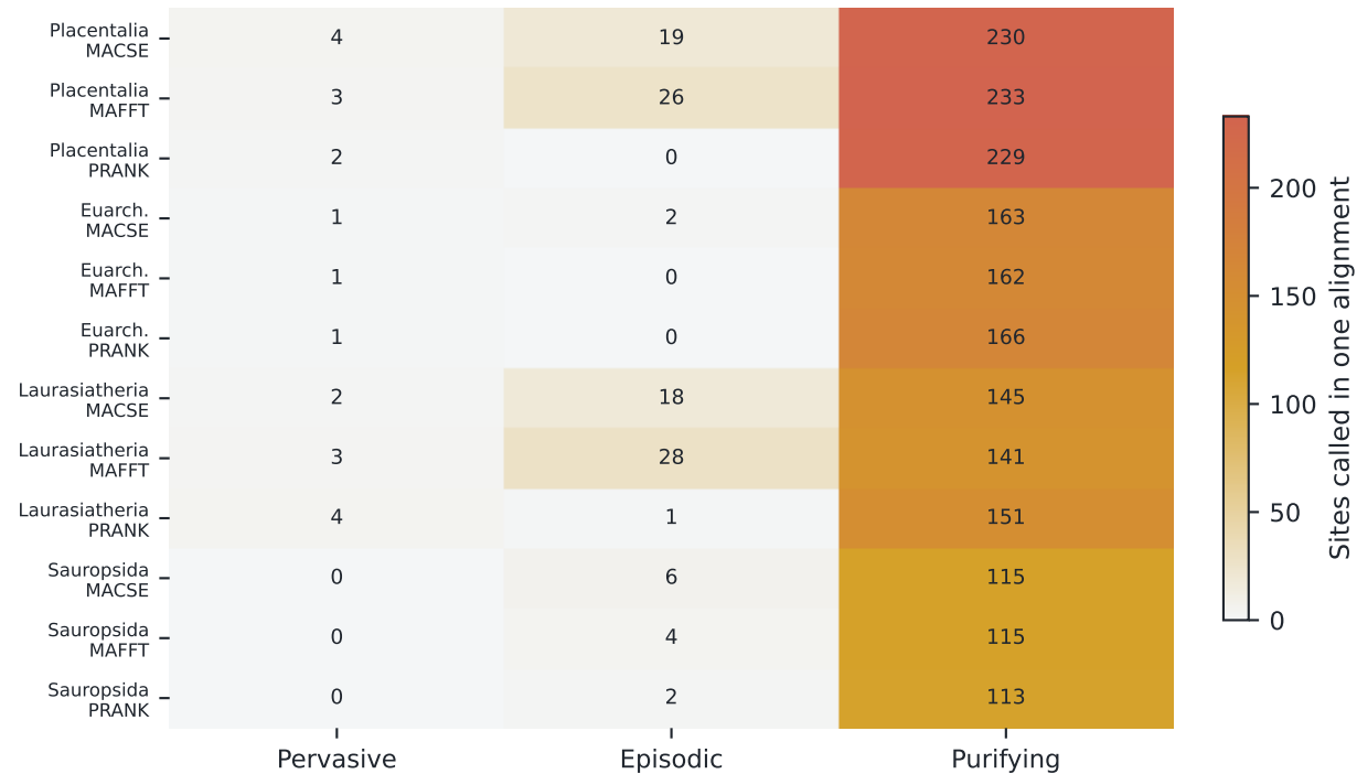
d Alignment and tree sensitivity
