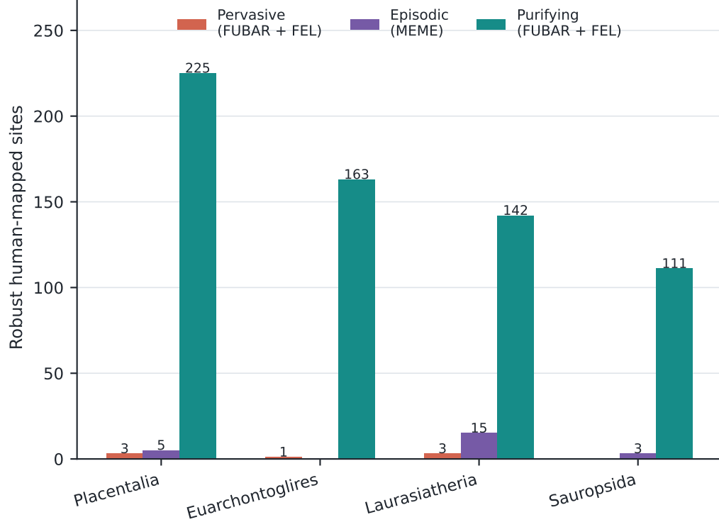
c h358 evidence across scopes and aligners
