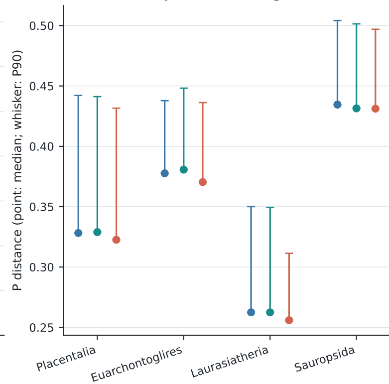
c Third-codon-position divergence
