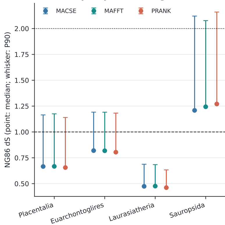
a Pairwise synonymous divergence
