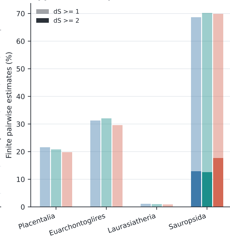
b Upper-tail multiple-hit indicators
