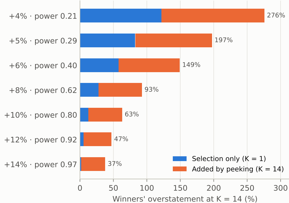
F4b · Peeking adds most of it, even at high power
