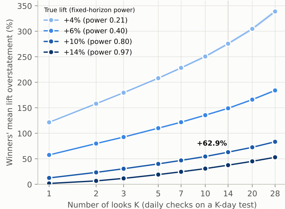
F4a · Declared winners overstate the design lift by +62.9% at K = 14
