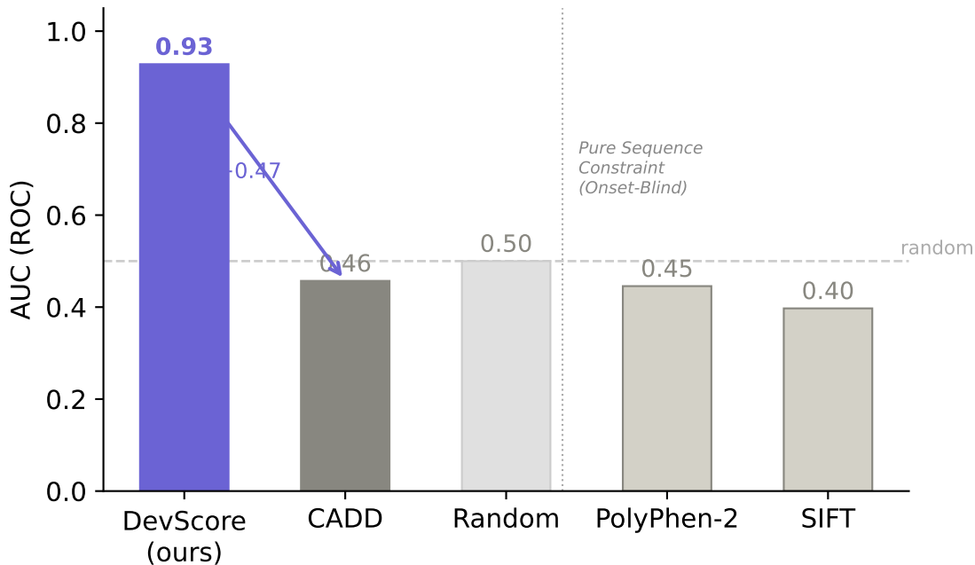
Fig. 1 — AUC comparison: developmental disease classification DevScore achieves AUC=0.93 vs primary comparator CADD (AUC=0.46)
