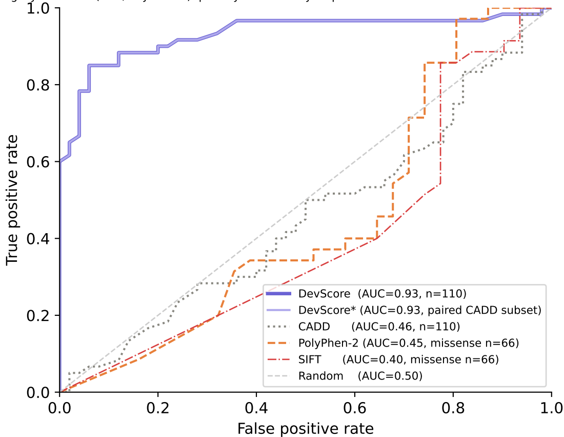
Fig. 2 — ROC curves: developmental disease classification Legacy baselines (SIFT/PolyPhen-2) quantify evolutionary sequence constraint rather than disease onset timing.
