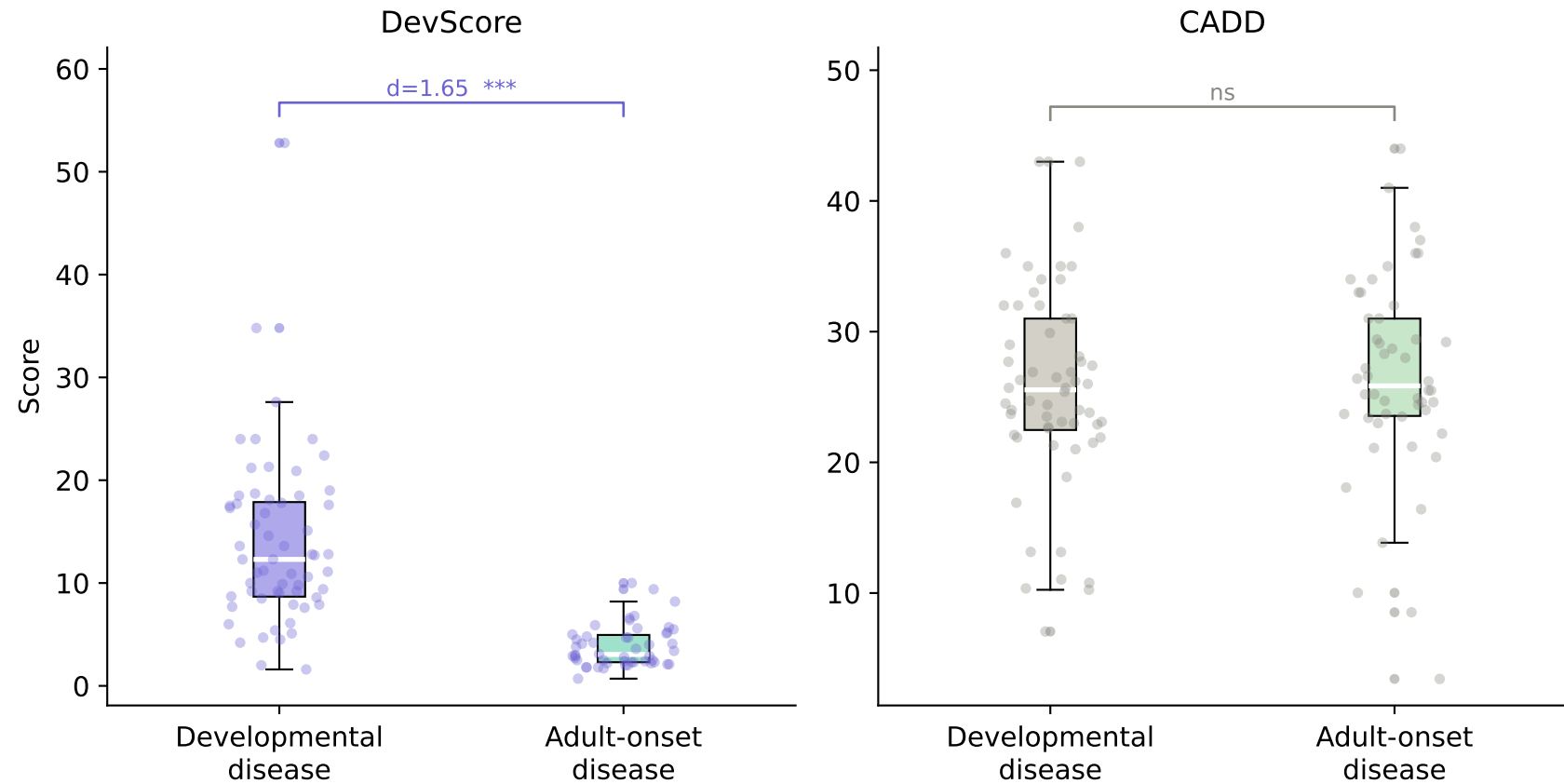
Fig. 3 — Score distributions by gene class
