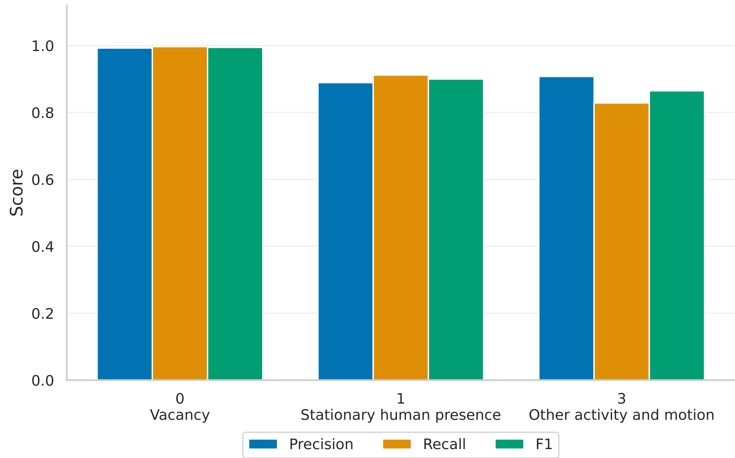
Per-Class Performance — RandomForest (CV mean)
