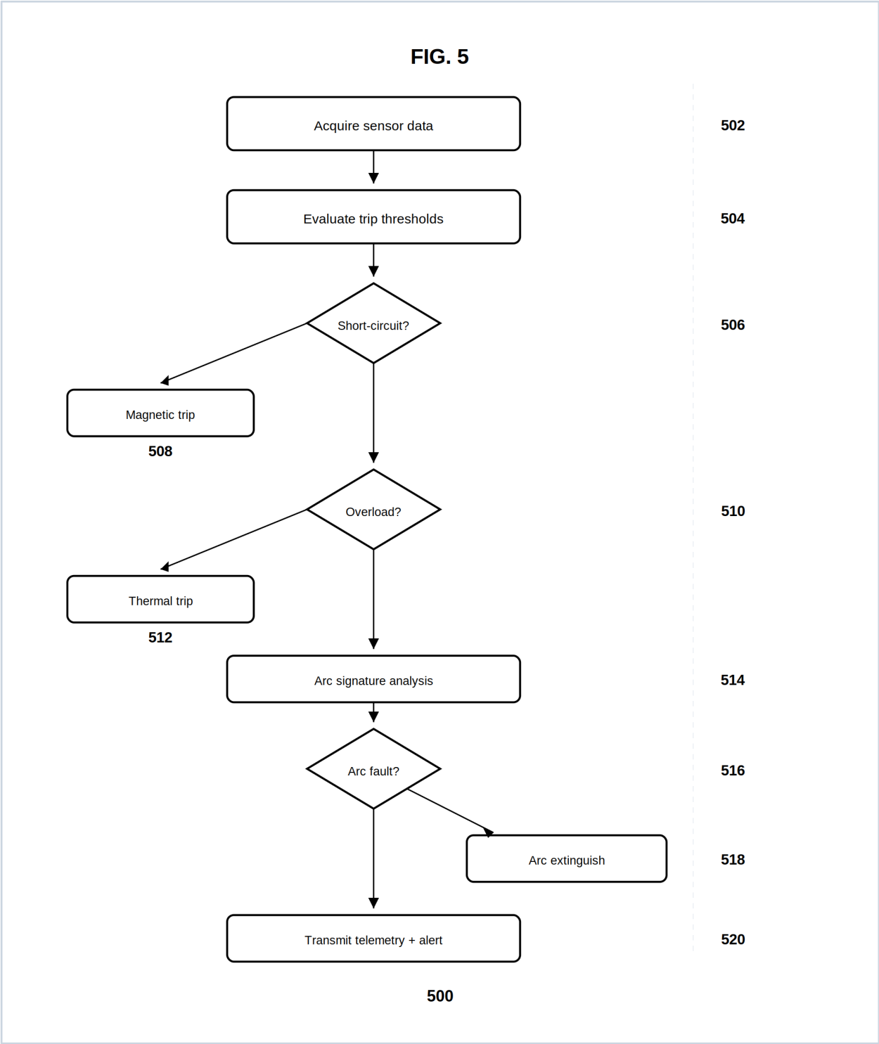
FIG. 5 - Process (500): acquisition, threshold evaluation, tripping, arc analysis, extinguishing, alert transmission.
