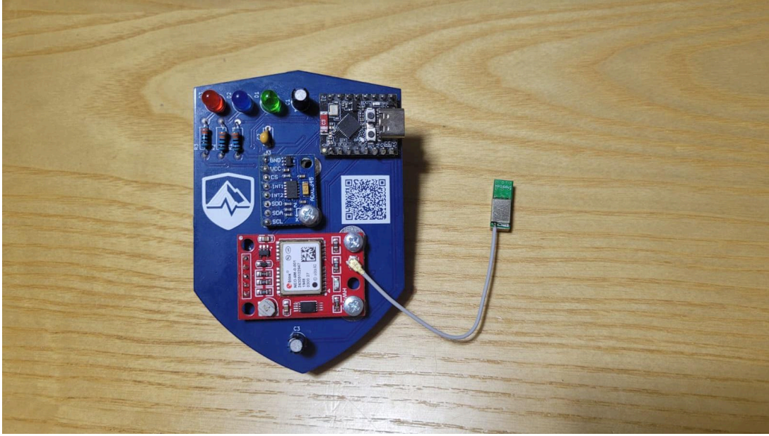
Figure 3.1: The QuakeGuard v2.0.0 fully assembled PCB, featuring the ESP32-C3 SuperMini, the ADXL345 accelerometer, and the u-blox GNSS module soldered into their dedicated footprints.
