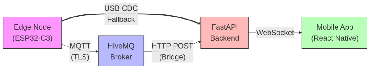
Figure 1: High-Level Architecture Block Diagram
