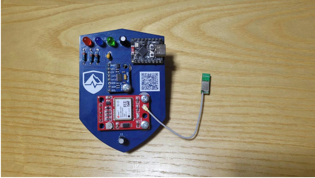
Figure 2: The QuakeGuard v2.0.0 fully assembled PCB, featuring the ESP32-C3 SuperMini, the ADXL345 accelerometer, and the u-blox GNSS module soldered into their dedicated footprints.
