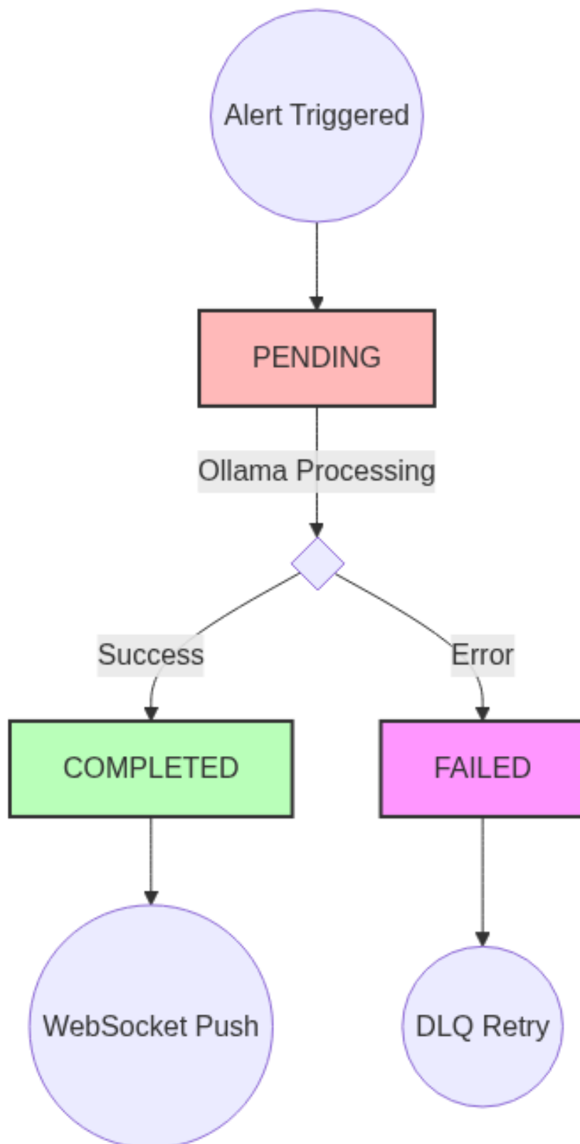
Figure 5: AI Report State Machine
