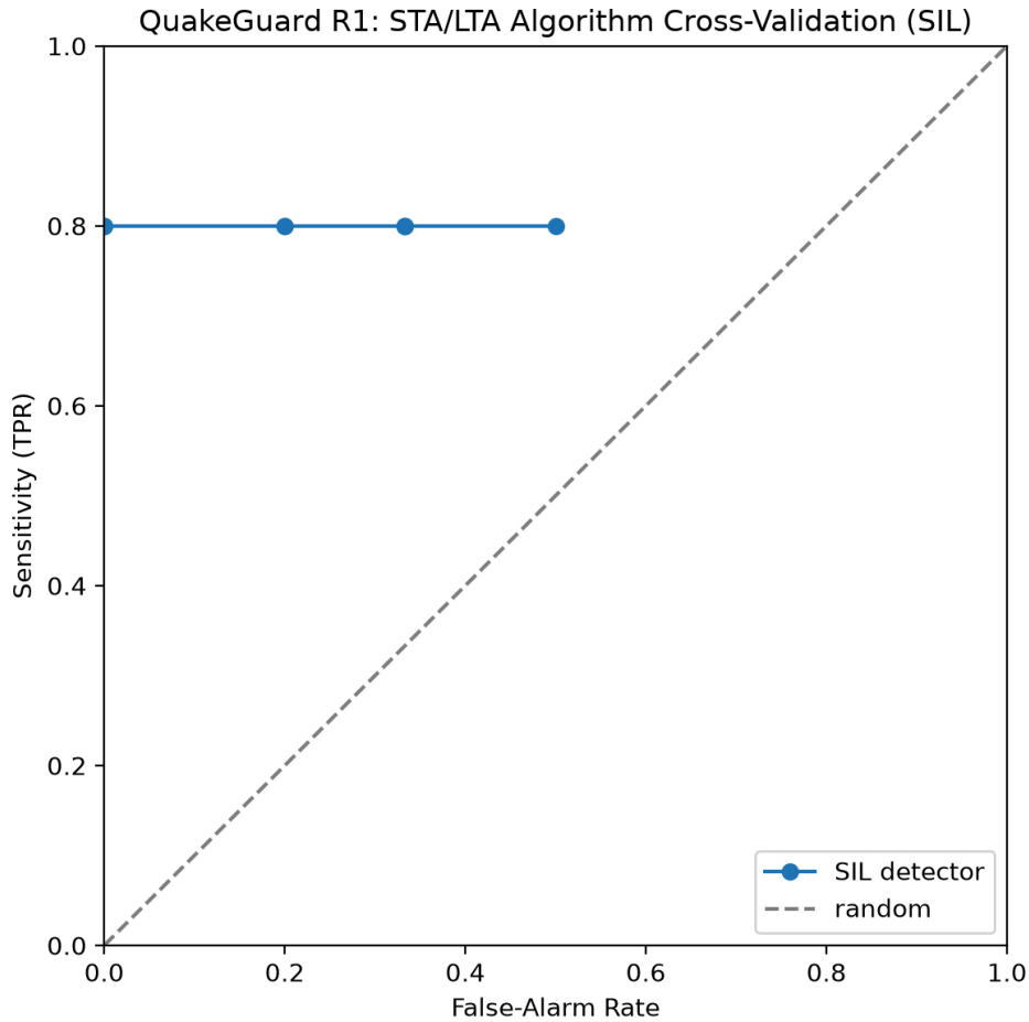
Figure 3: Receiver Operating Characteristic (ROC) curve of the edge STA/LTA algorithm. The curve reaches a hard upper bound at 0.8 (80%) True Positive Rate (Sensitivity). This limit represents a highly desirable geophysical outcome: 4 out of 5 historical events are perfectly identified without any false alarms (FAR = 0.0), while the 5th event (a weak micro-seismicity recorded at >100km distance) correctly fails to trigger the algorithm, proving the firmware's robustness against distant noise.
