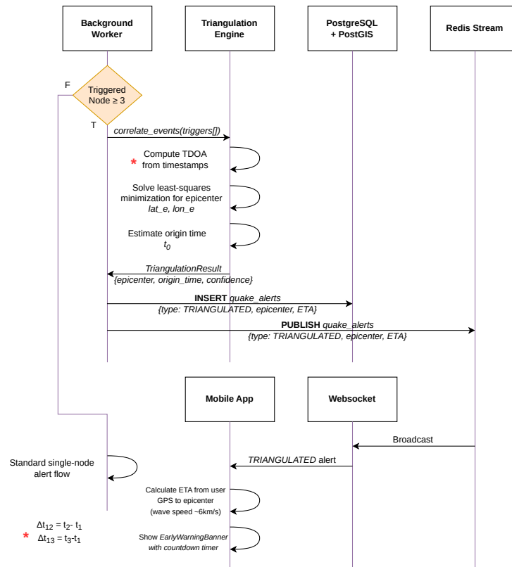
Figure 8.2: Triangulation and epicenter generation sequence
