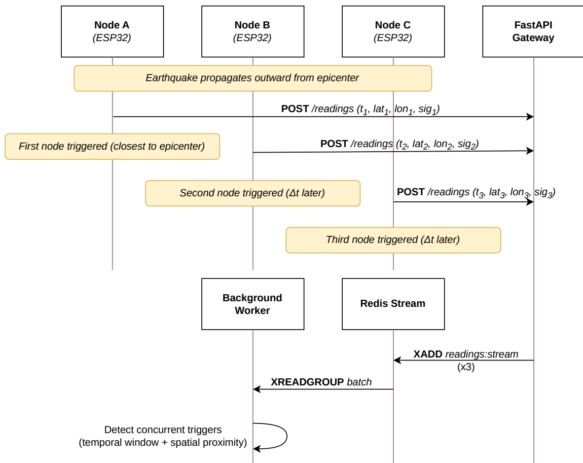
Figure 9.1: Temporal and spatial clustering sequence for seismic triggers
