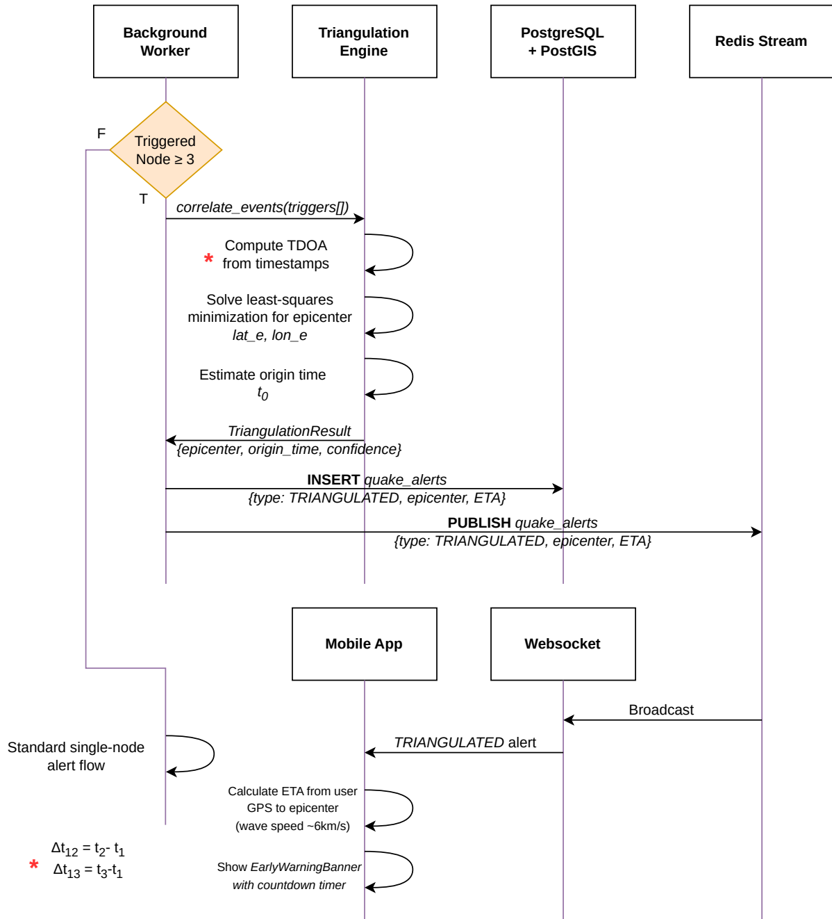
Figure 9.2: Triangulation and epicenter generation sequence
