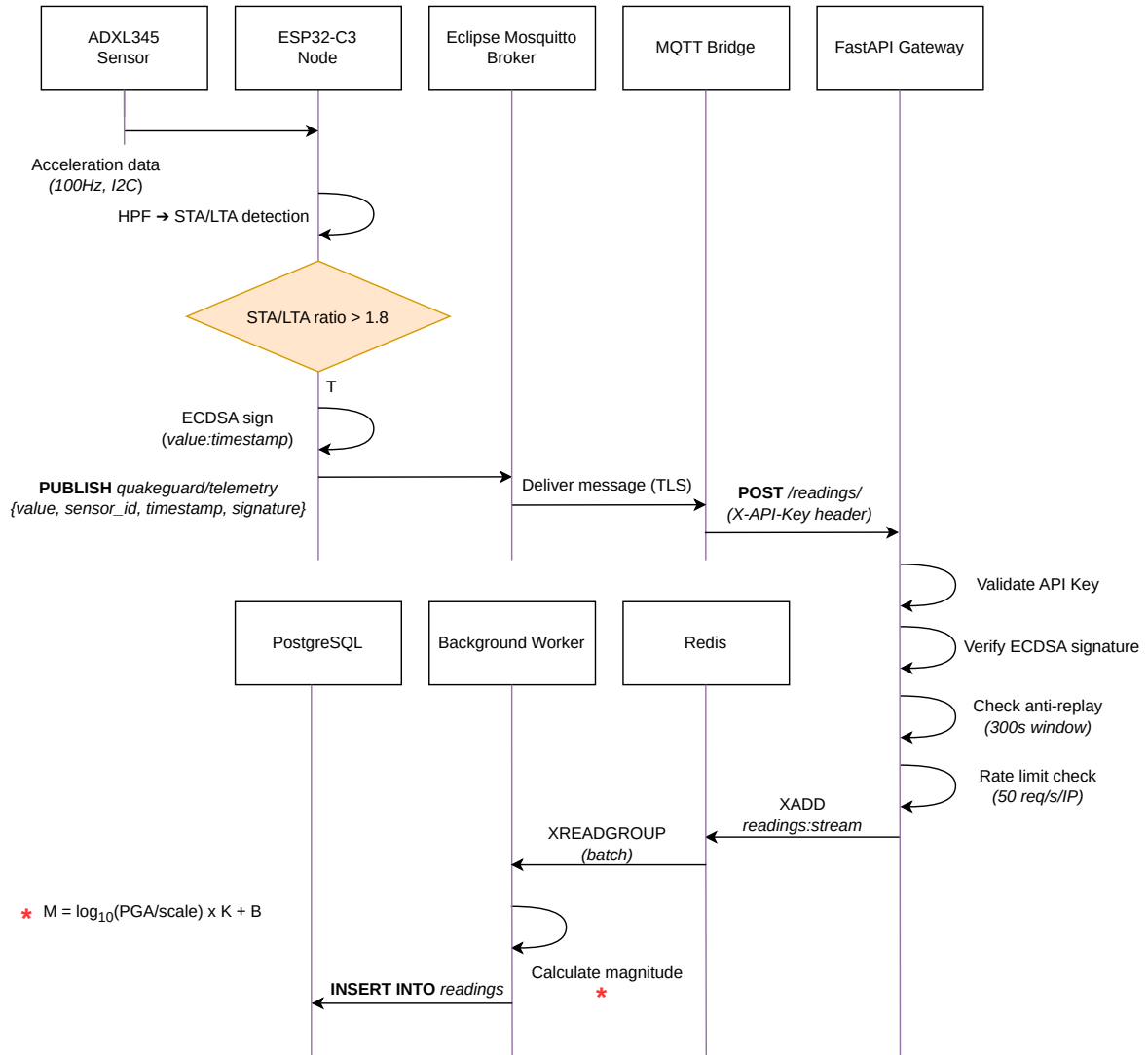
Figure 6.1: Telemetry ingestion and magnitude estimation sequence
