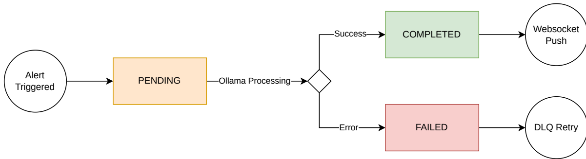
Figure 8: AI Report State Machine
