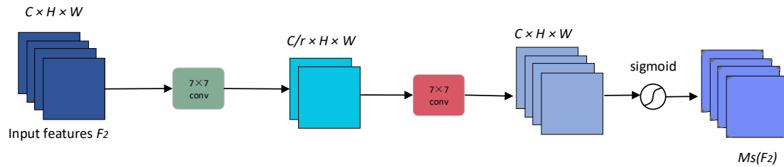
Figure 3. The structure of spatial attention module.
