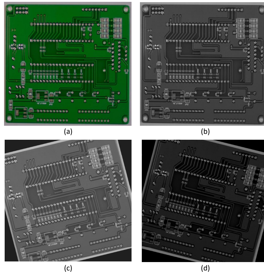
Figure 8. The processing of image enhancement. (a) The original image. (b) The grayscale-processed image. (c) The image rotated 15 degrees to the right with brightness increased by 15%. (d) The image rotated 15 degrees to the left with brightness decreased by 15%.
