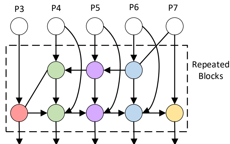
Figure 6. The BiFPN structure.
