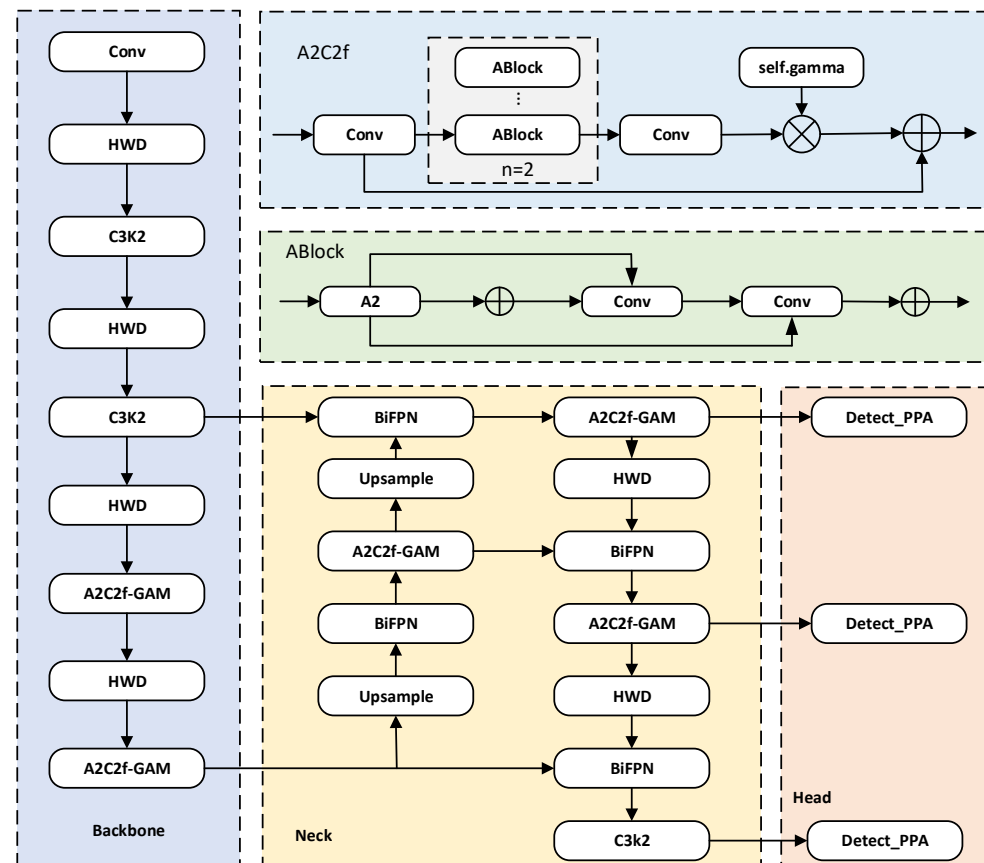
Figure 1. The enhanced YOLOv12 network architecture with multi-module fusion.
