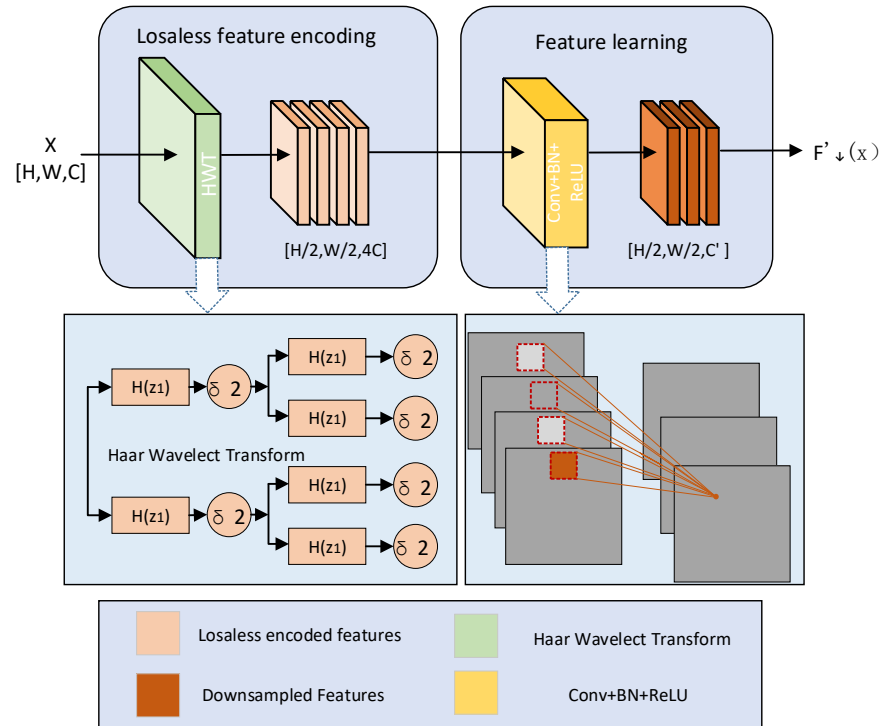
Figure 5. The HWD module architecture.
