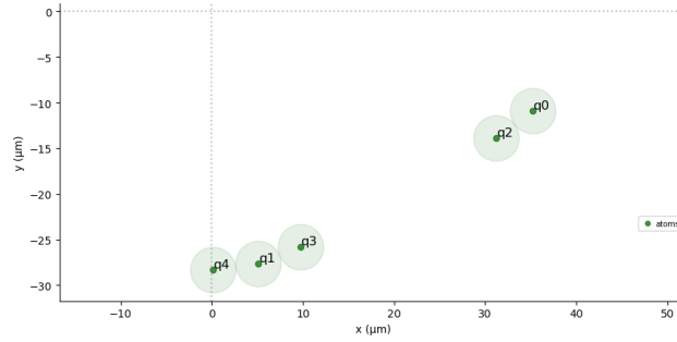
Figure 3.5: The optimal 2D physical spatial layout generated by the Genetic Algorithm for the N = 5 instance. The register fully complies with Neutral Atom QPU geometric boundaries.
