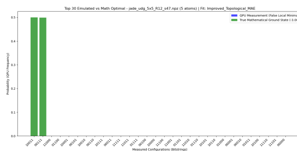
Figure 3.6: Probability distribution of the measured bitstrings after the adiabatic execution on the QPU emulator. The highest probability peaks correspond perfectly to the optimal solutions of the original QUBO instance.
