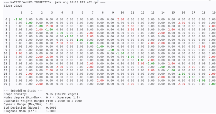
Figure 5.7: Structure of the 20 \times 20 UDG-like QUBO instance generated via instance_generator.py , inspected using inspect_qubo.py , and subsequently embedded using the bench-SA.py module [26].
