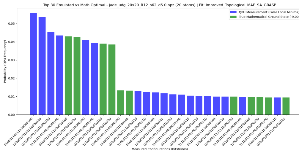
Figure 5.12: Probability distribution of the measured bitstrings after the adiabatic execution on the QPU emulator. While noisy, the system managed to identify at least one optimal solution of the original QUBO instance.
