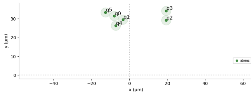
Figure 4.5: The 2D physical spatial layout generated by the Genetic Algorithm for the N = 6 instance. The register fully complies with Neutral Atom QPU geometric boundaries.
