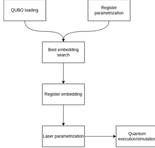
Figure 3.1: Flowchart of the basic pipeline. The process highlights an hybrid classical-quantum approach.
