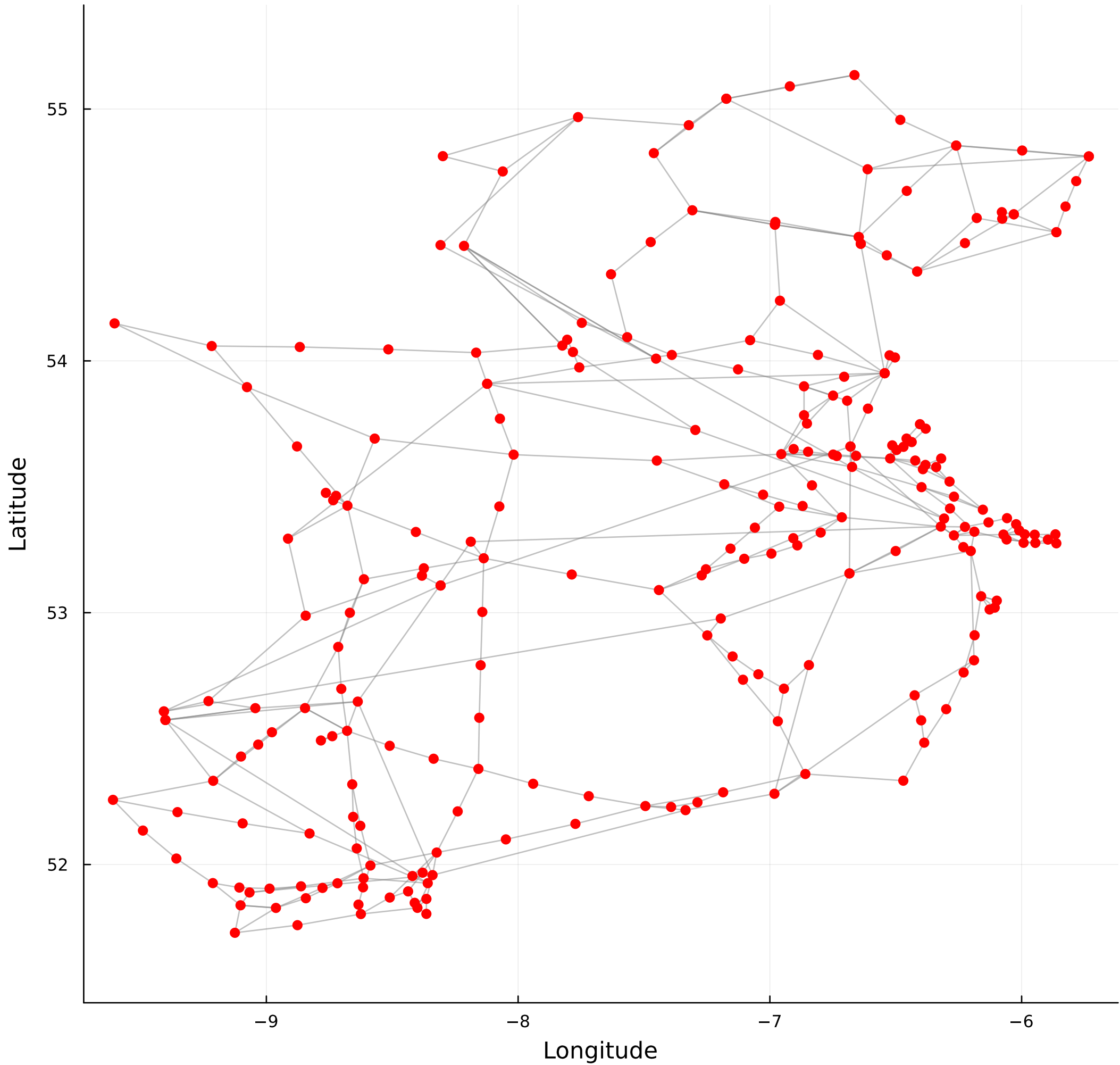
Irish Electricity Grid
