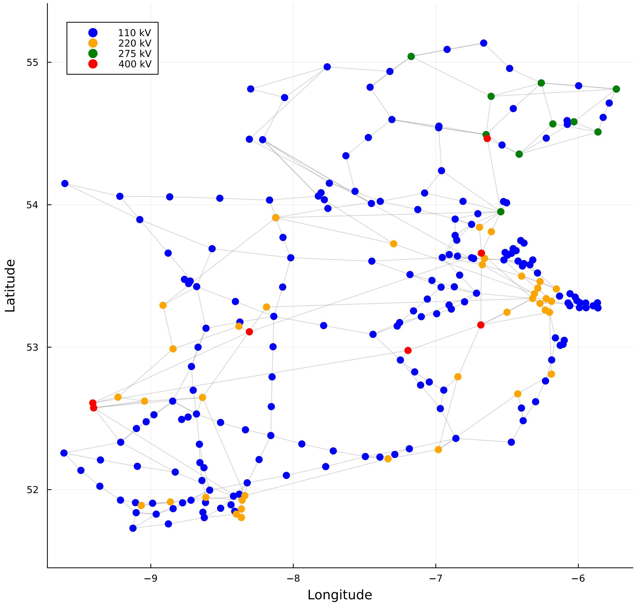
Irish Electricity Grid - Colored by Voltage Level
