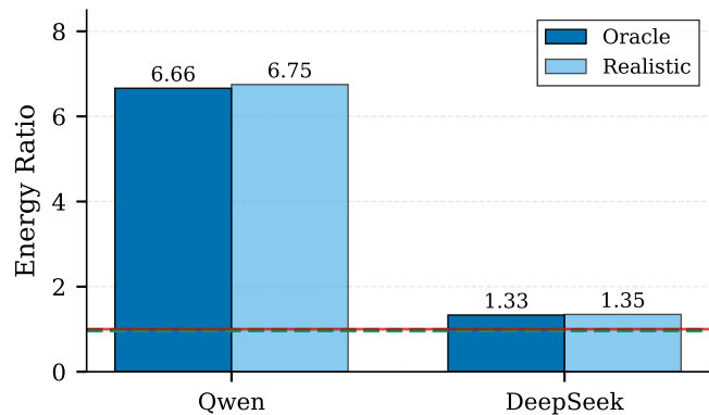
(b) Oracle vs Realistic Context
