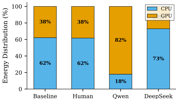
(c) CPU vs GPU Energy Share
