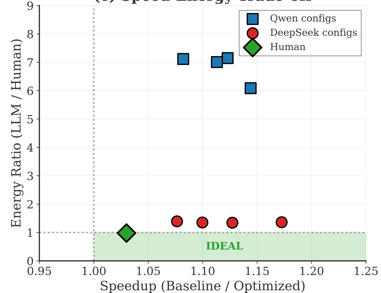
(c) Speed-Energy Trade-off
