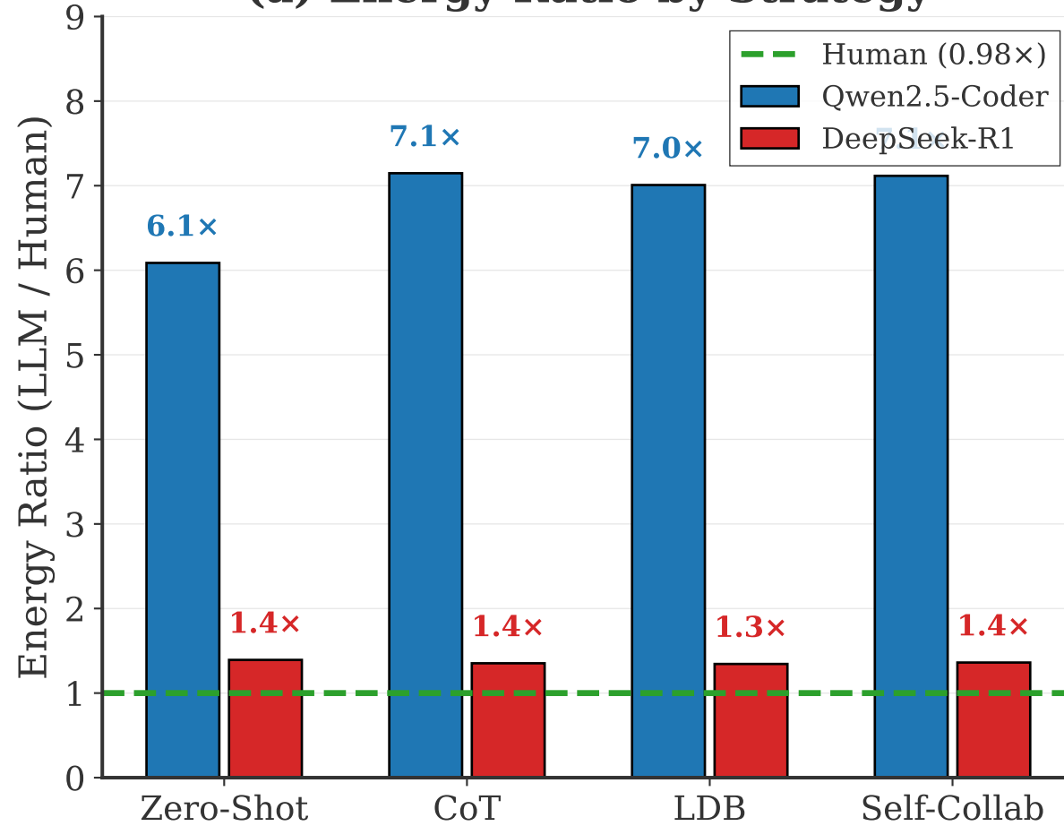
(a) Energy Ratio by Strategy
