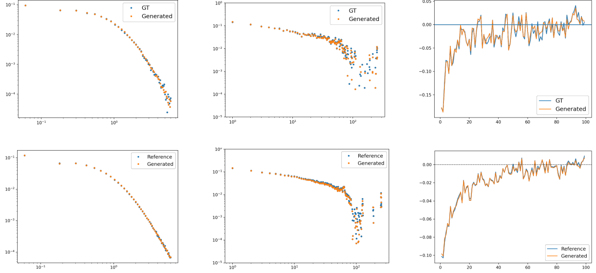
Figure 6.10: Stylized facts with Reference or Ground Truth (GT) (blue) versus Generated for the EDM-CSDI (Cond.) model. Top row : validation windows only; first column : Validation windows versus the ground truth (conditioning windows). second column : combined validation and training windows versus the entire Reference (dataset). Left column : heavy-tail distribution; centre column : volatility clustering; right column : leverage effect.
