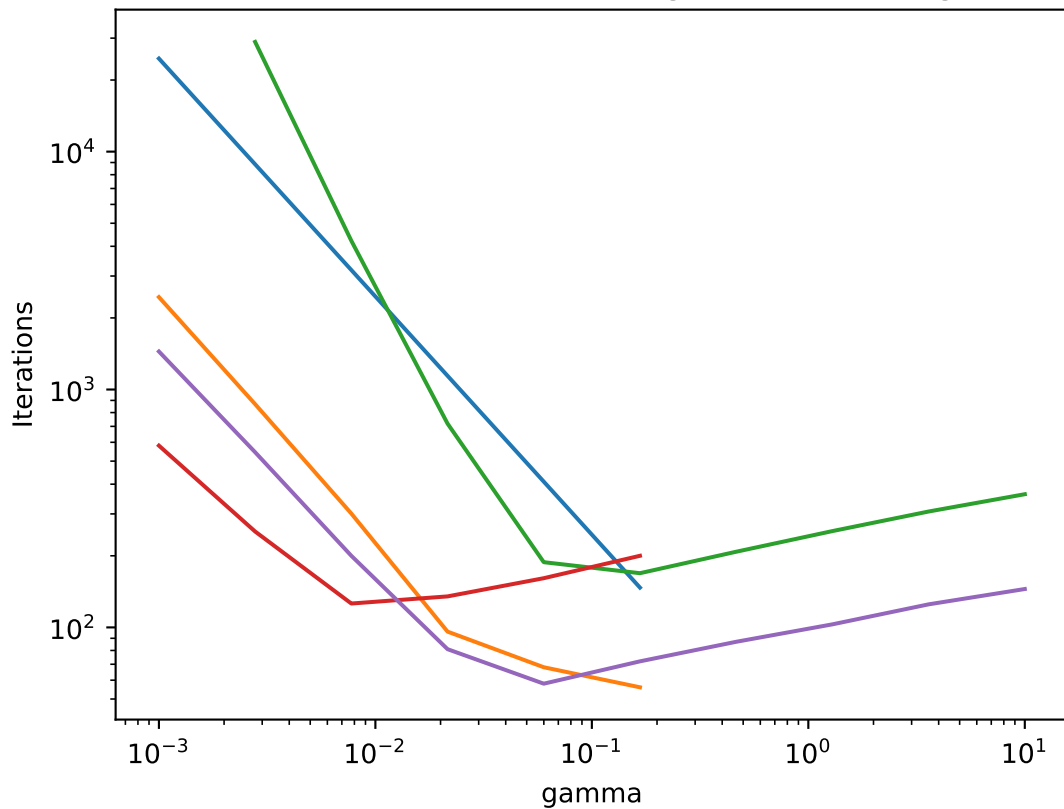
Iterations needed for convergence 1e-02, Ridge
