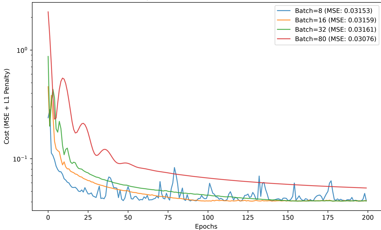
Lasso Optimization: Batch GD vs. Stochastic GD
