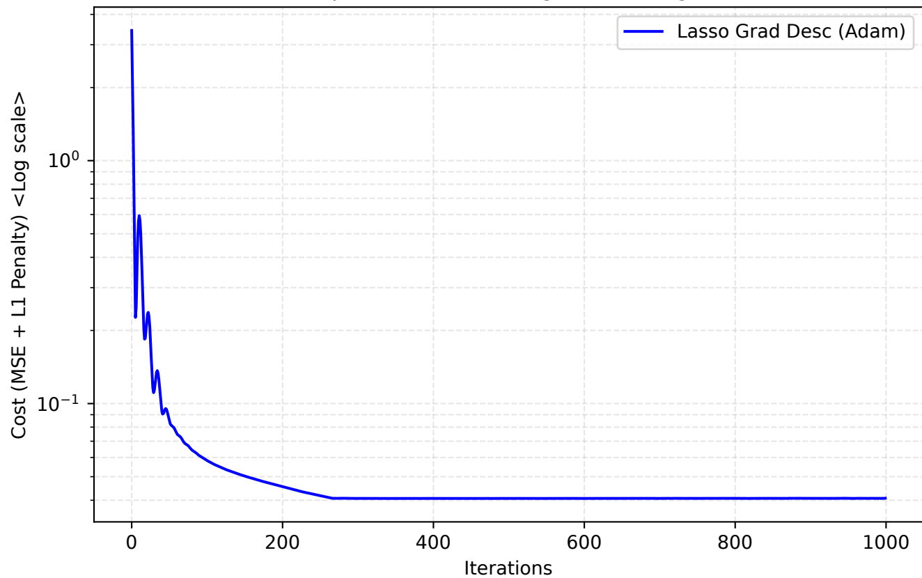
Lasso Optimisation learning curve <Log scale>
