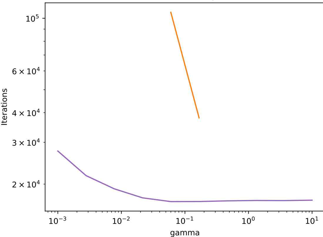
Iterations needed for convergence 1e-02, OLS
