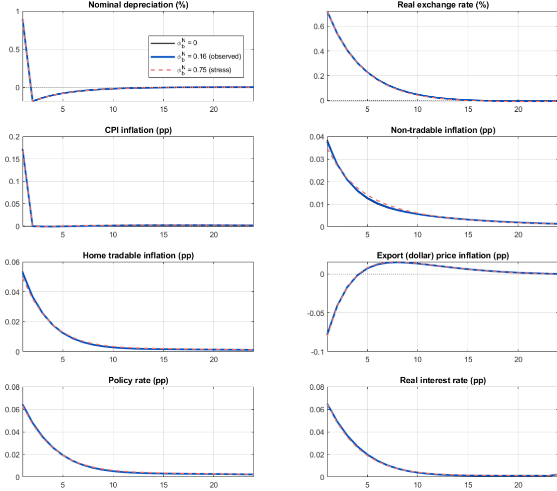
Figure 8: Baseline financial tightening: prices and monetary policy. Responses to a 25bp foreign interest-rate tightening at \phi_b^N \in \{0, 0.16, 0.75\} and \phi_b^T = 0.28 . Exchange rates are percent deviations from steady state; inflation and interest rates are in quarterly percentage points. The real interest rate is r_t^H - \mathbb{E}_t \pi_{t+1} . The near-coincidence of the three paths shows that changing non-tradable debt dollarization leaves the aggregate price and policy block nearly unchanged.
