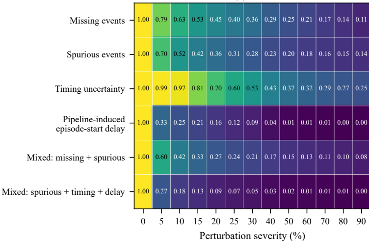
(a) TEP
