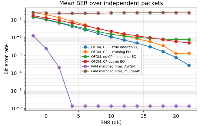
Fig. 6. Mean bit error rate versus SNR over 20 independent packet trials. CP-OFDM with one-tap equalization improves with SNR, while single-carrier matched filtering without equalization has an ISI-driven error floor in the multipath channel.
