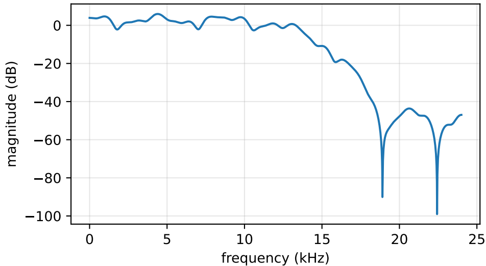
Simulated speaker-room-microphone response
