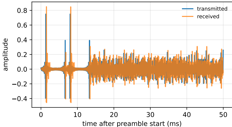
Audio OFDM packet through simulated loopback
