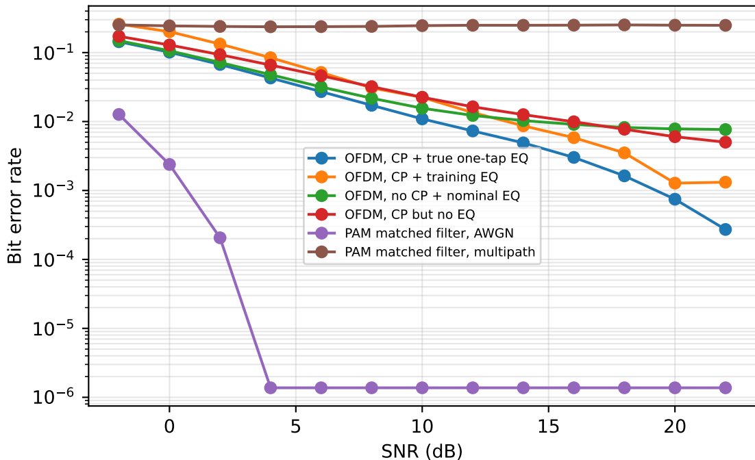
Mean BER over independent packets
