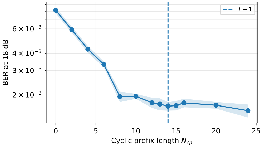
BER penalty when the cyclic prefix is too short
