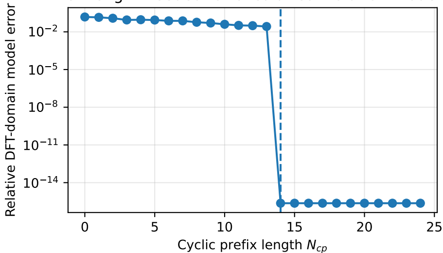
CP length needed for circular convolution model
