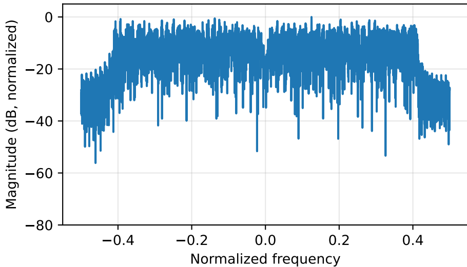
OFDM baseband spectrum
