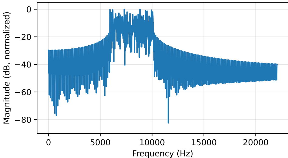
Real passband OFDM audio packet spectrum
