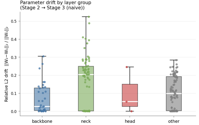
Figure 4: Relative L2 parameter drift (Stage 2 → Stage 3, naive) per layer group, restricted to the learnable (gradient-updated) tensors. The neck adapts most (median \approx 0.20 ) and the backbone least (median \approx 0.03 ); the three detection-head tensors show only modest drift (median \approx 0.05 ). Excluding the BatchNorm running-statistic buffers removes the spurious head-layer drift seen when all parameters are pooled, the gradient-updated head weights barely move, consistent with starvation of the absent large-target stratum rather than active overwriting of the output layers.
