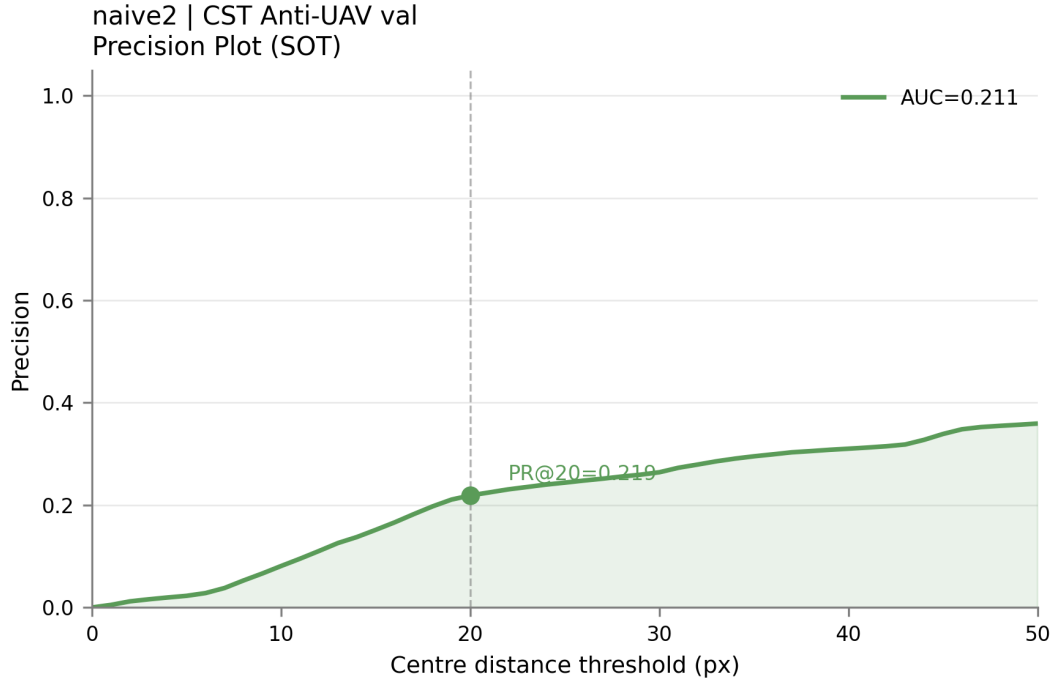
Figure 8: Precision plot on CST Anti-UAV validation set (Stage 3 best checkpoint, epoch 3). The representative score at threshold 20 px (PR@20) is reported in the main tracking evaluation table.
