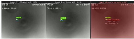
Figure 5: Detection output on the same Anti-UAV-RGBT validation frame (sequence 20190925_101846, clip 1_4, frame 0) under three successive checkpoints. Left: Stage 1 best checkpoint (T1 ceiling, mAP@0.5 = 0.6725). Centre: Stage 2 best checkpoint after knowledge distillation (mAP@0.5 = 0.640, FM = -0.033). Right: Stage 3 naive fine-tuning at epoch 3 (T1 mAP@0.5 = 0.068, FM = -0.605); the absence of large-target detections is in line with the gradient-starvation interpretation discussed above.
