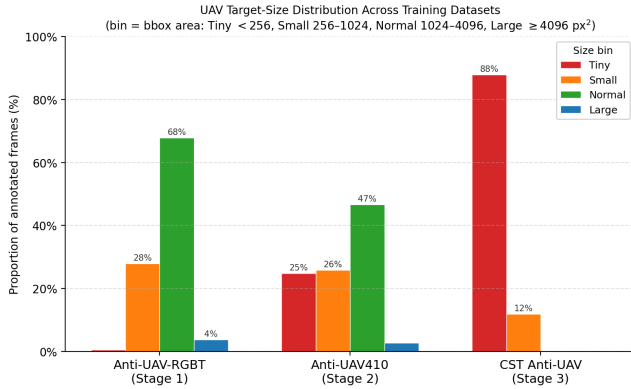
Figure 1: Scale distribution across the three training datasets (train + val splits, bbox area: tiny <256 \text{ px}^2 , small 256\text{--}1024 \text{ px}^2 , normal 1024\text{--}4096 \text{ px}^2 , large \geq 4096 \text{ px}^2 ). Anti-UAV-RGBT is dominated by normal targets (67.8%; 95.8% normal or small). CST Anti-UAV shows a near-complete inversion: 87.9% tiny; 99.8% tiny or small.
