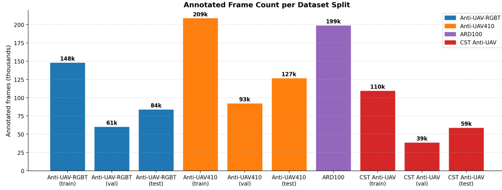
Figure 6: Per-split counts of UAV-present frames—frames in which a UAV is present (the exist=1 flag), labelled ‘annotated’ on the figure axis. Anti-UAV410 is the largest (428,703 across train/val/test), followed by Anti-UAV-RGBT (293,209). CST Anti-UAV (208,221) and ARD100 (199,291) are comparable in size; ARD100 is used only for motion-mask pre-computation and is not part of the continual learning curriculum.
