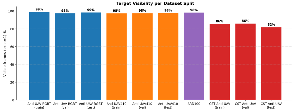
Figure 7: Target visibility per dataset split. A frame is marked visible if it contains an actively flying UAV (the exist=1 flag); occluded or out-of-frame instances are marked absent. Anti-UAV-RGBT has the highest visibility rate, CST Anti-UAV the lowest, consistent with the difficulty of detecting sub-16-pixel targets in cluttered thermal scenes.
