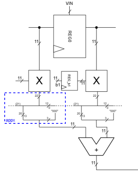
Figure 1.4: FIR architecture in details
