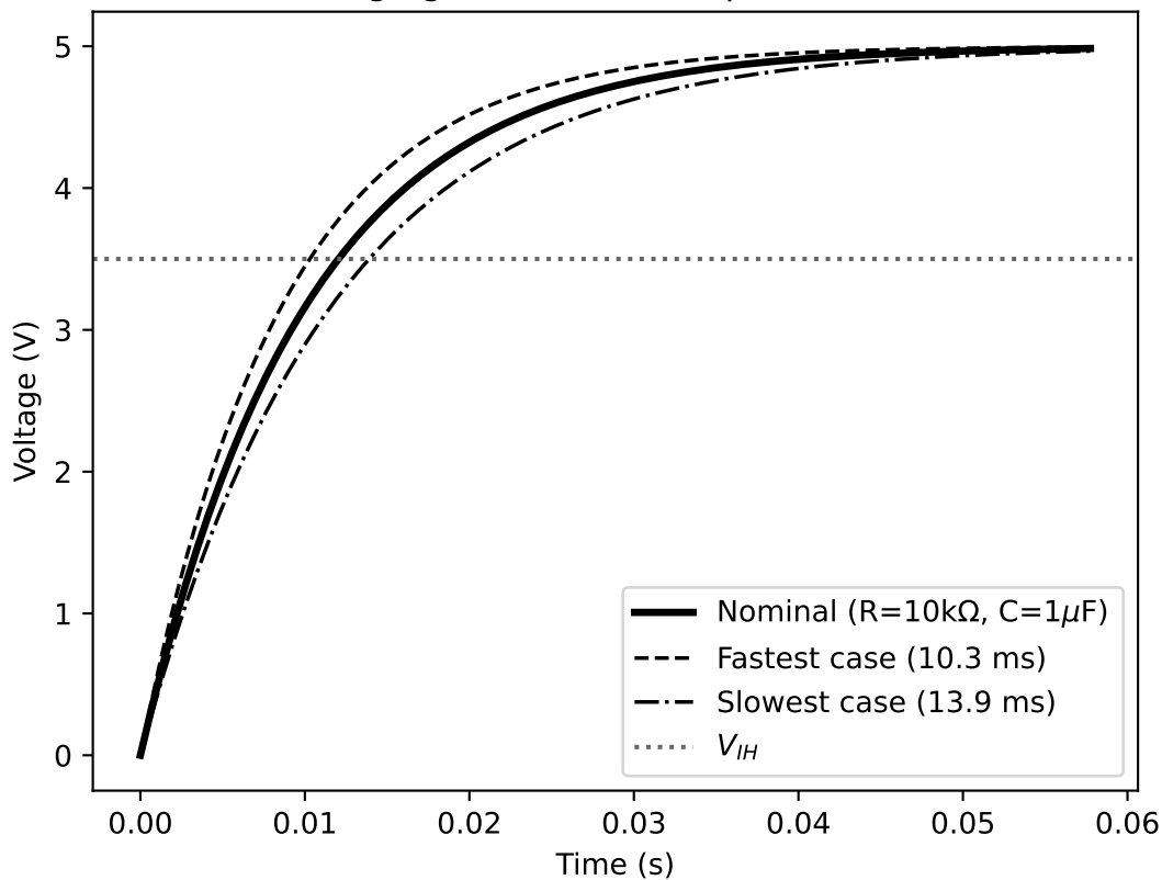
POR charging curve with component tolerance
