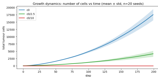
Our result
