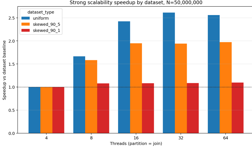
Figure 5: Strong-scaling speedup for the dedicated workload-balanced OpenMP executable.
