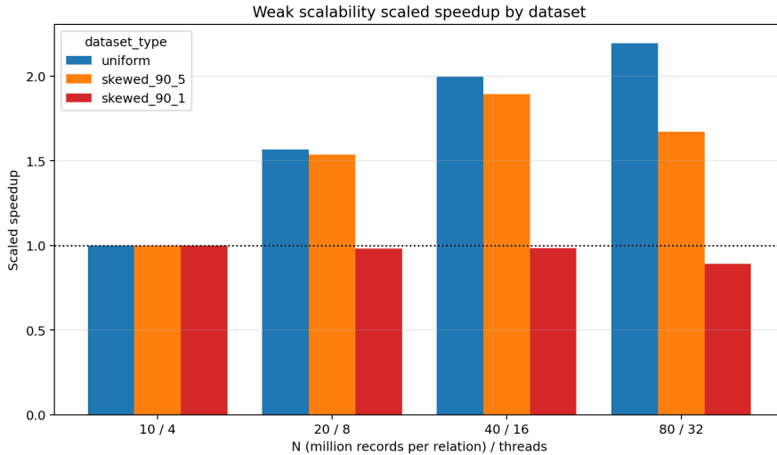
Figure 4: Weak-scaling scaled speedup for uniform and skewed datasets.
