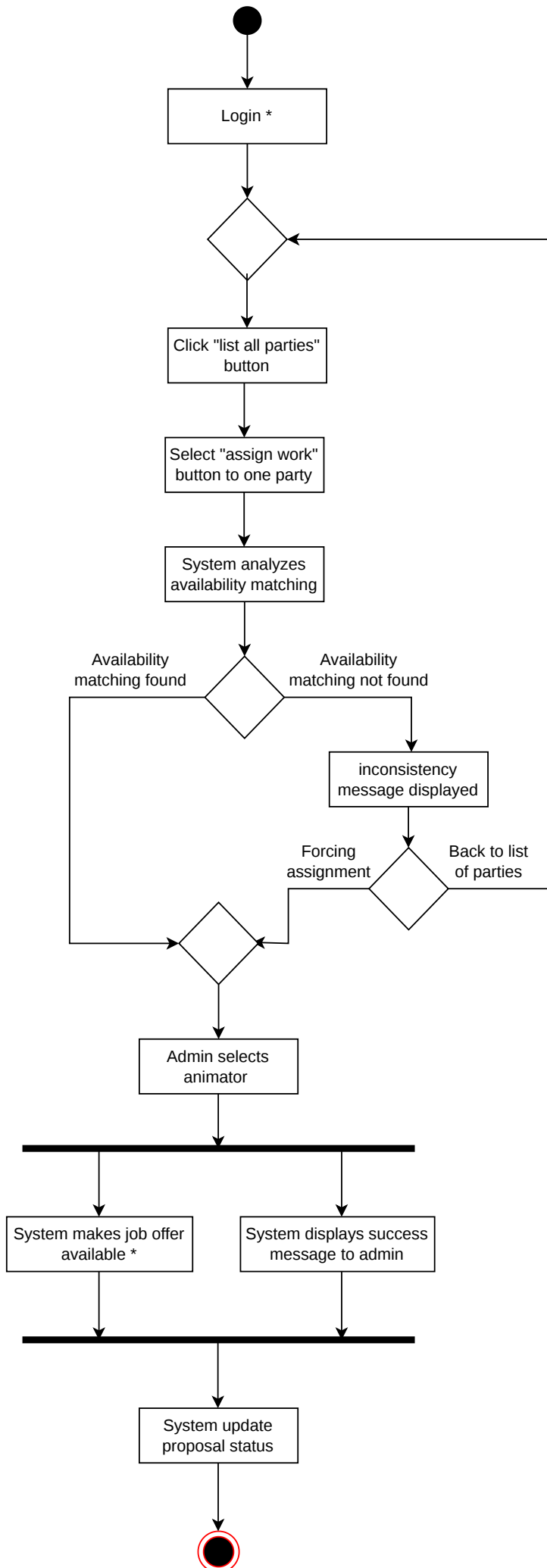
Activity Diagram: assign work to animator
