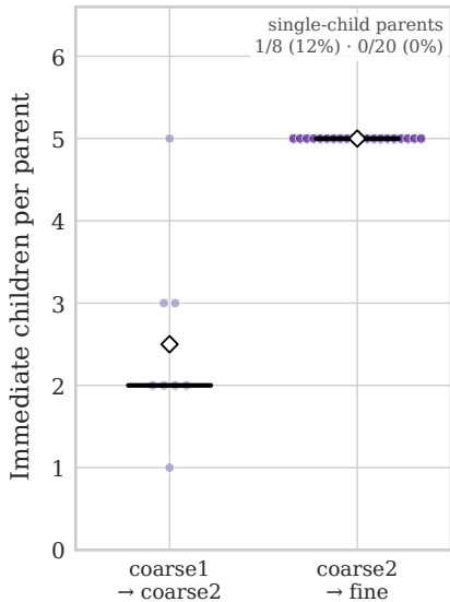
CIFAR-100
