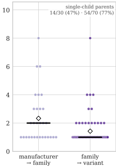
Aircraft
